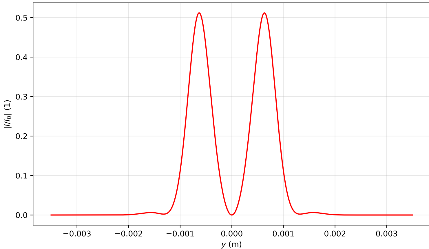
Intensity profile I(x=0, y, z=1.353)/I_0 , P_{in}=4.0P_{cr} , artificial time
